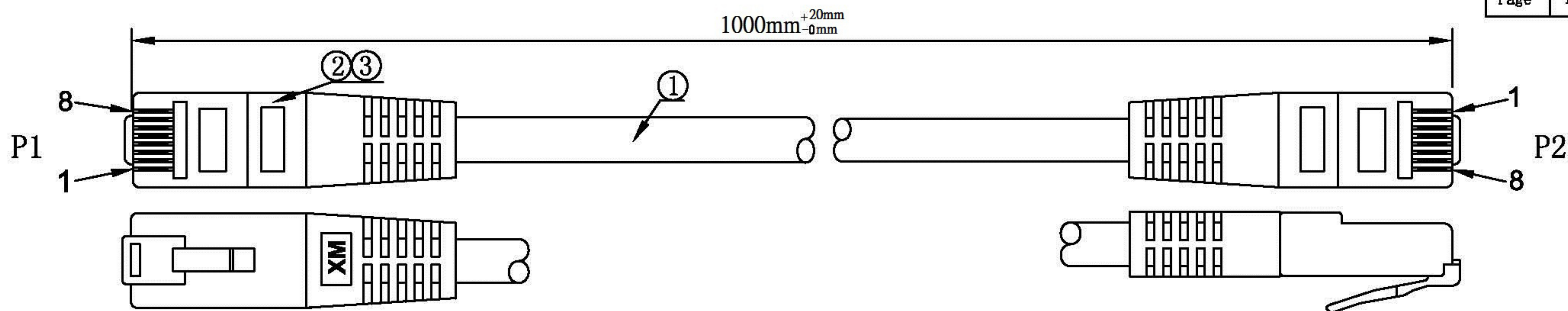
WIRING DIAGRAM
